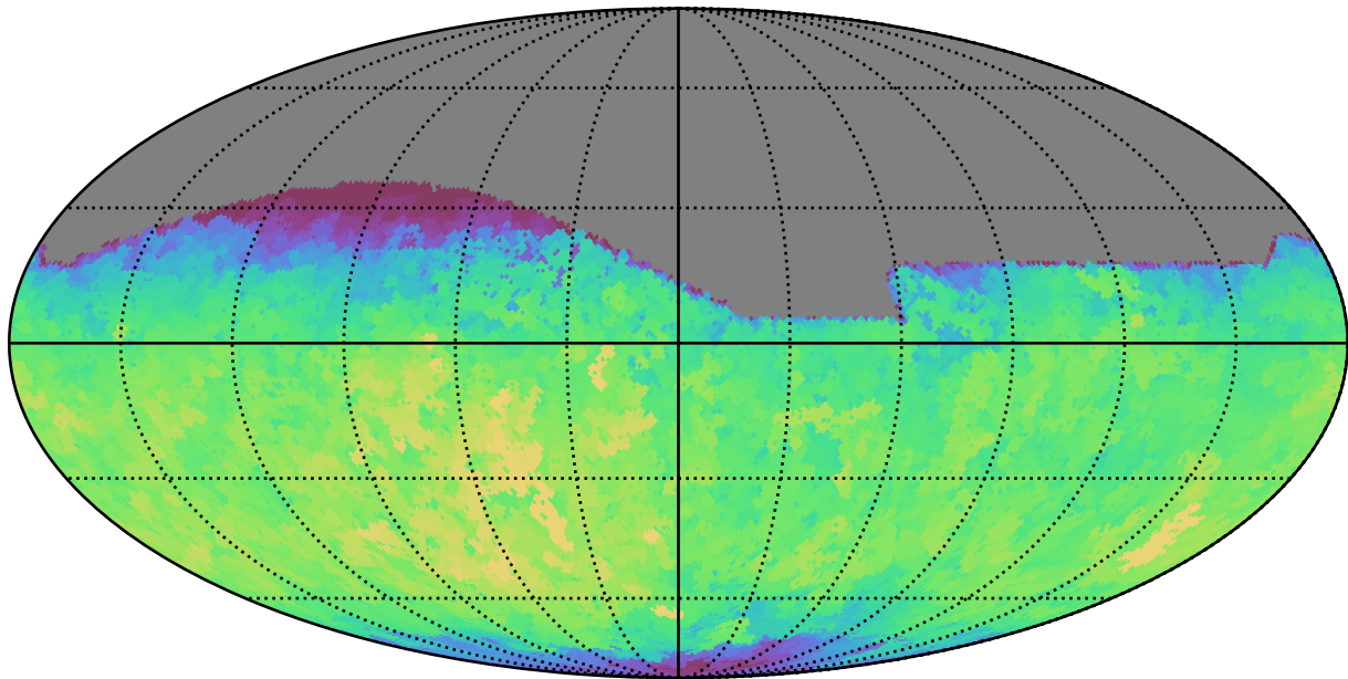
reweight_plane_v3.3_10yrs All sky g band: Max fiveSigmaDepth
