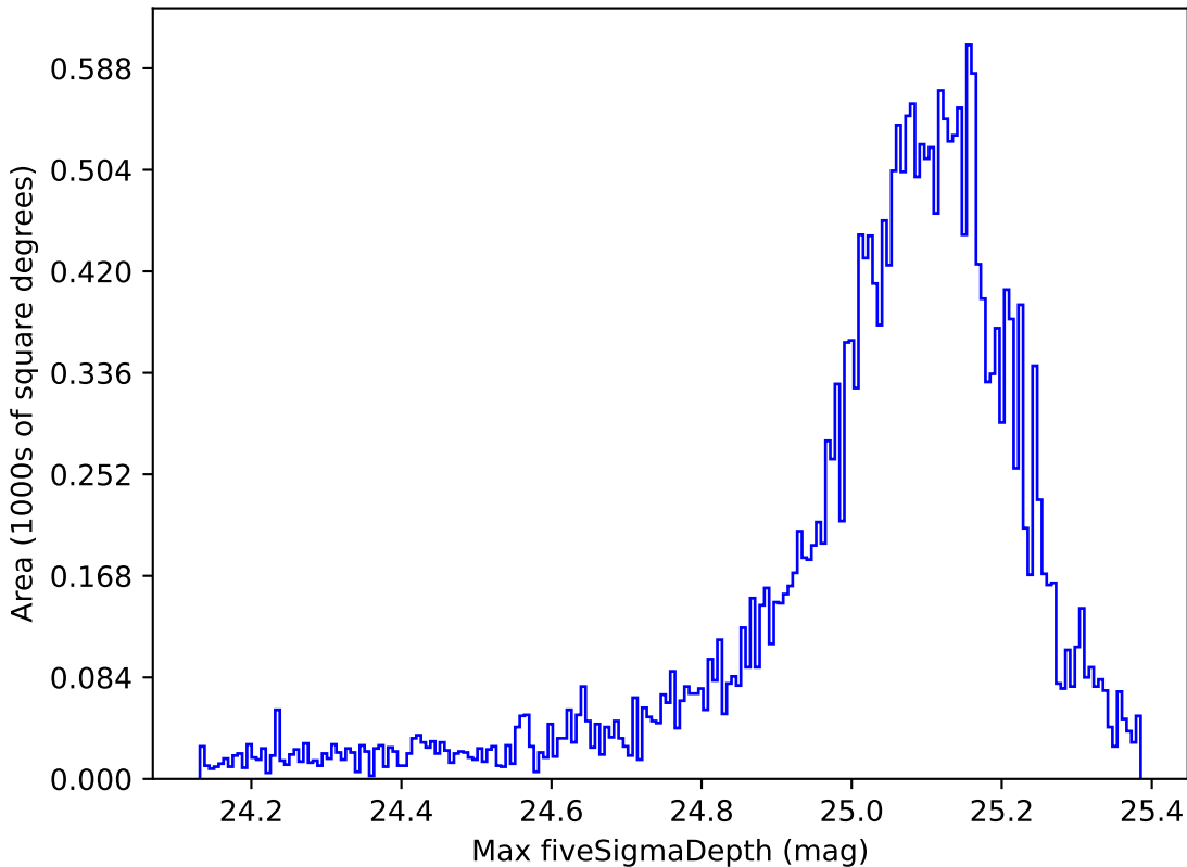
reweight_plane_v3.3_10yrs All sky all bands: Max fiveSigmaDepth
