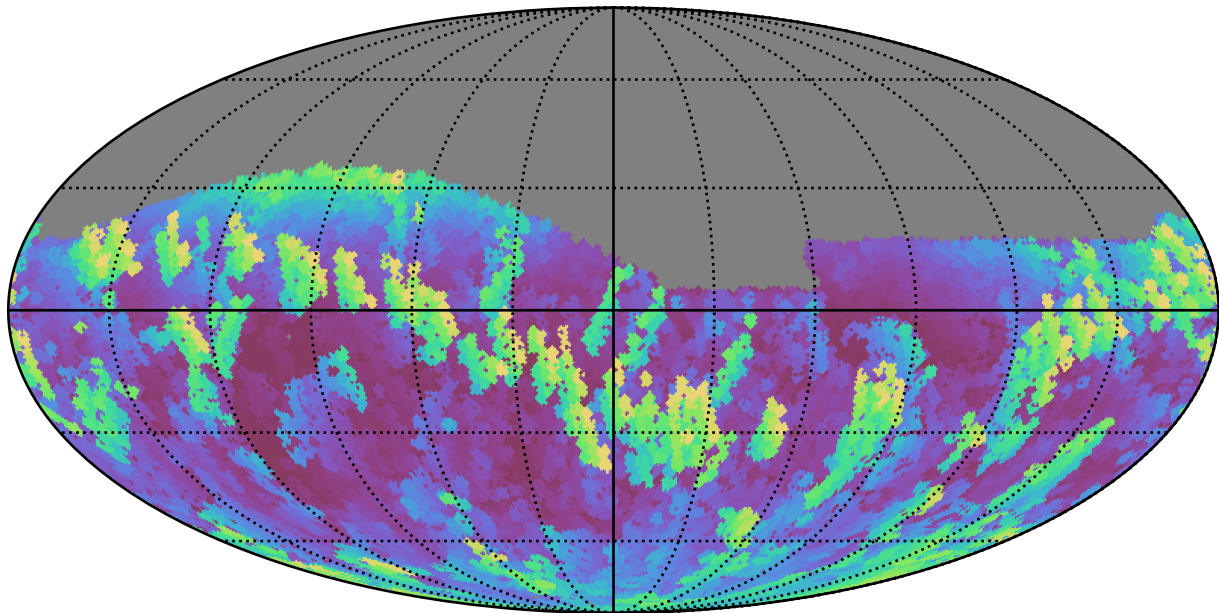
reweight_plane_v3.3_10yrs Yr 1 z band: Max airmass
