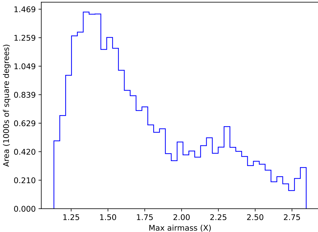
reweight_plane_v3.3_10yrs Yr 1 z band: Max airmass
