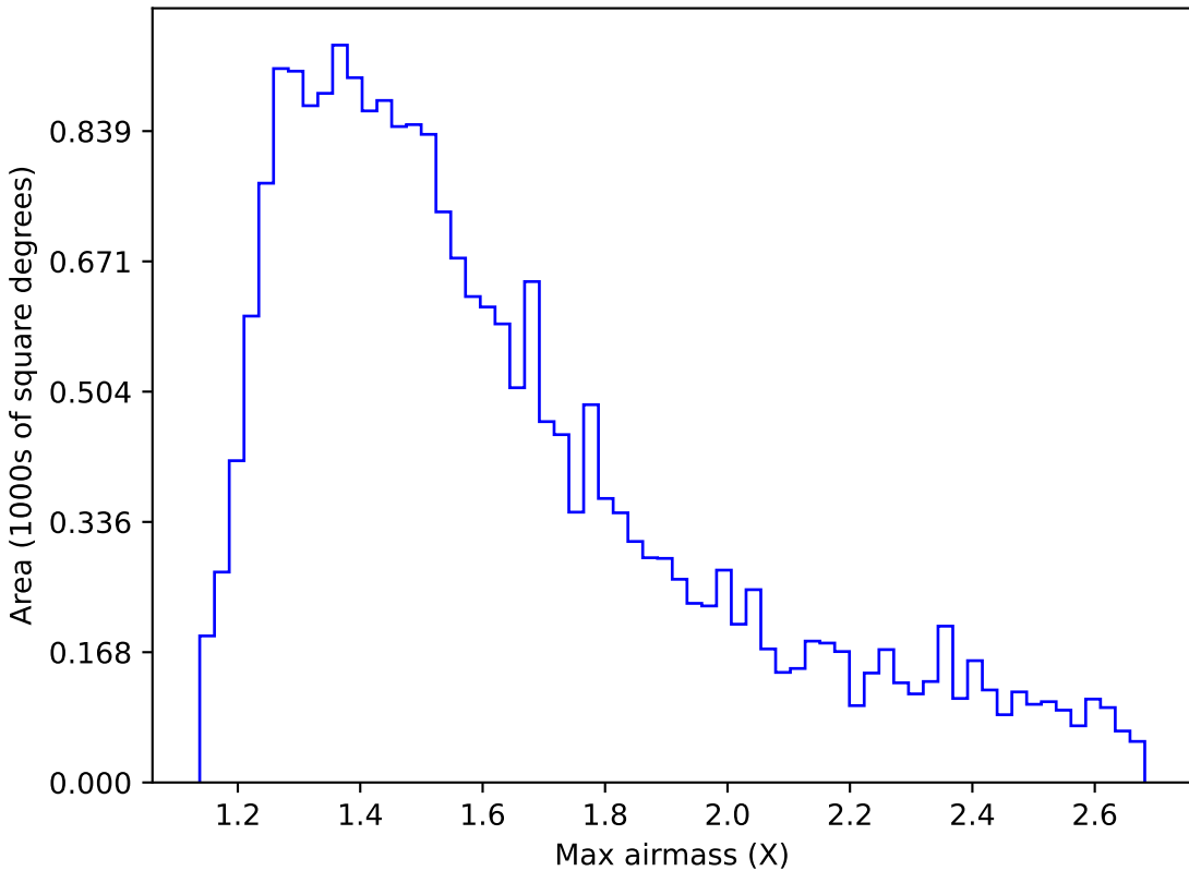
reweight_plane_v3.3_10yrs Yr 1 y band: Max airmass
