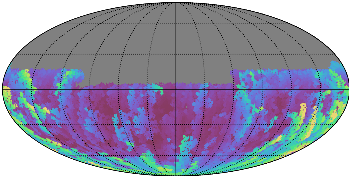
reweight_plane_v3.3_10yrs Yr 1 u band: Max airmass
