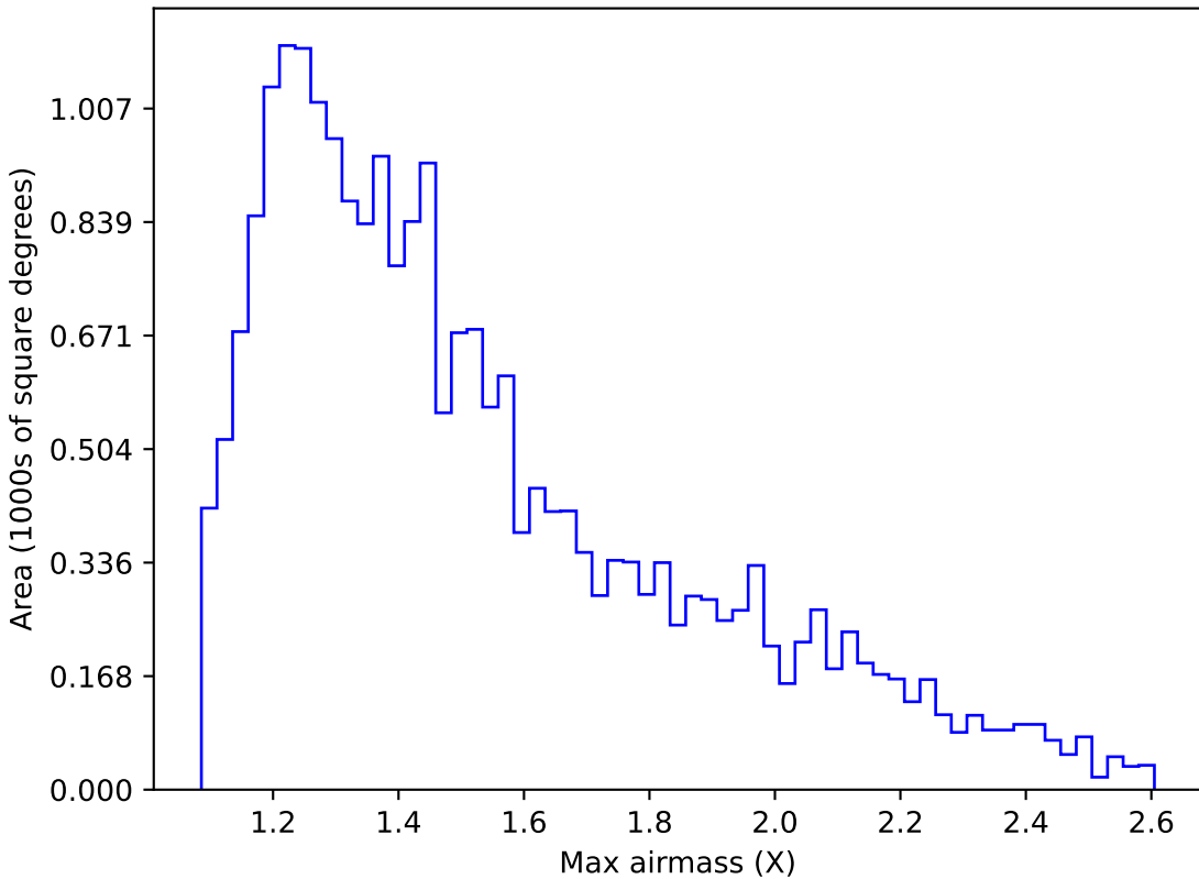
reweight_plane_v3.3_10yrs Yr 1 u band: Max airmass
