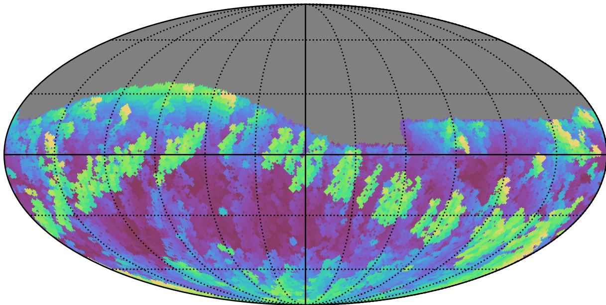
reweight_plane_v3.3_10yrs Yr 1 r band: Max airmass
