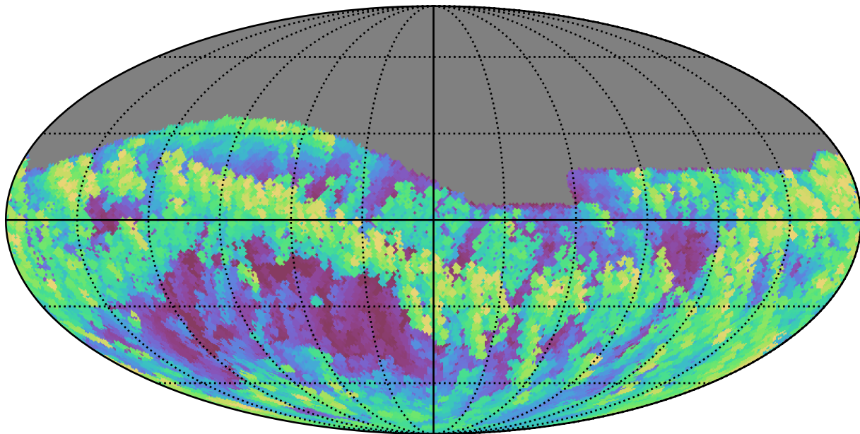
reweight_plane_v3.3_10yrs Yr 1 all bands: Max airmass
