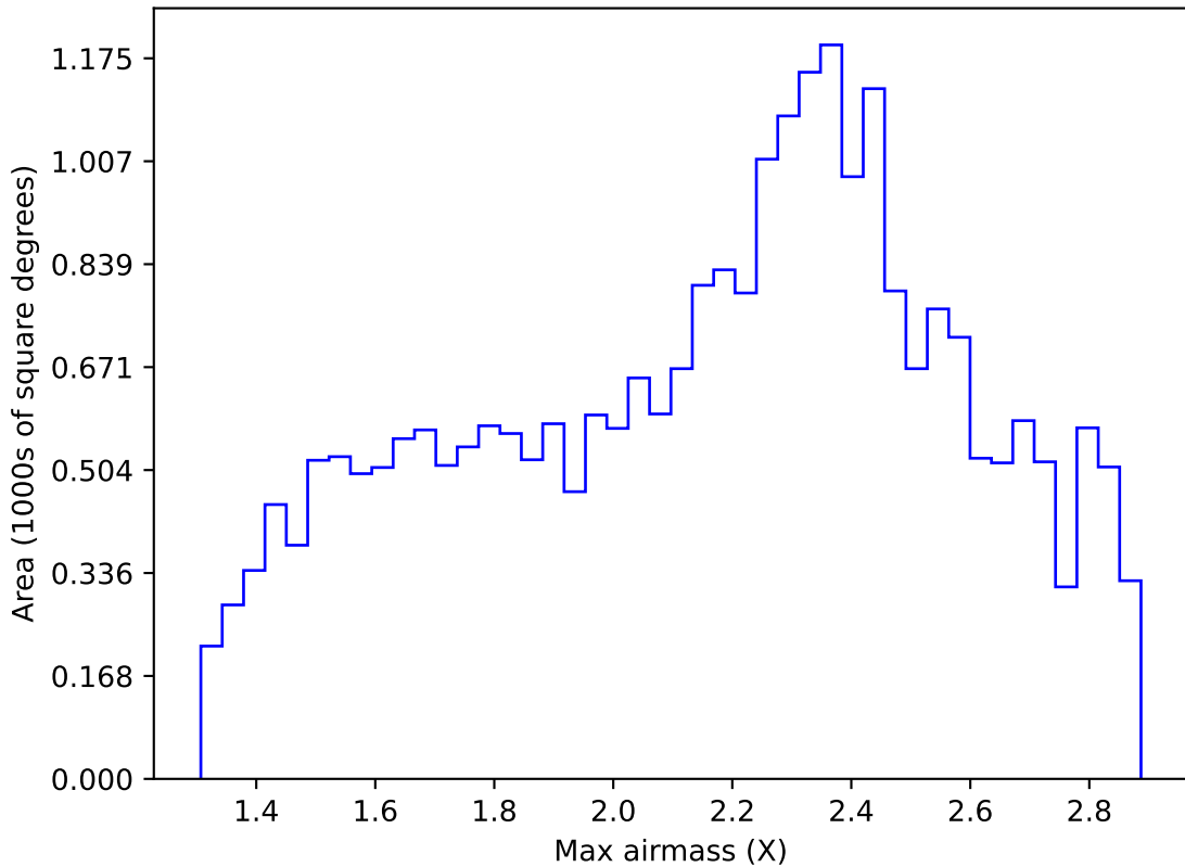
reweight_plane_v3.3_10yrs Yr 1 all bands: Max airmass
