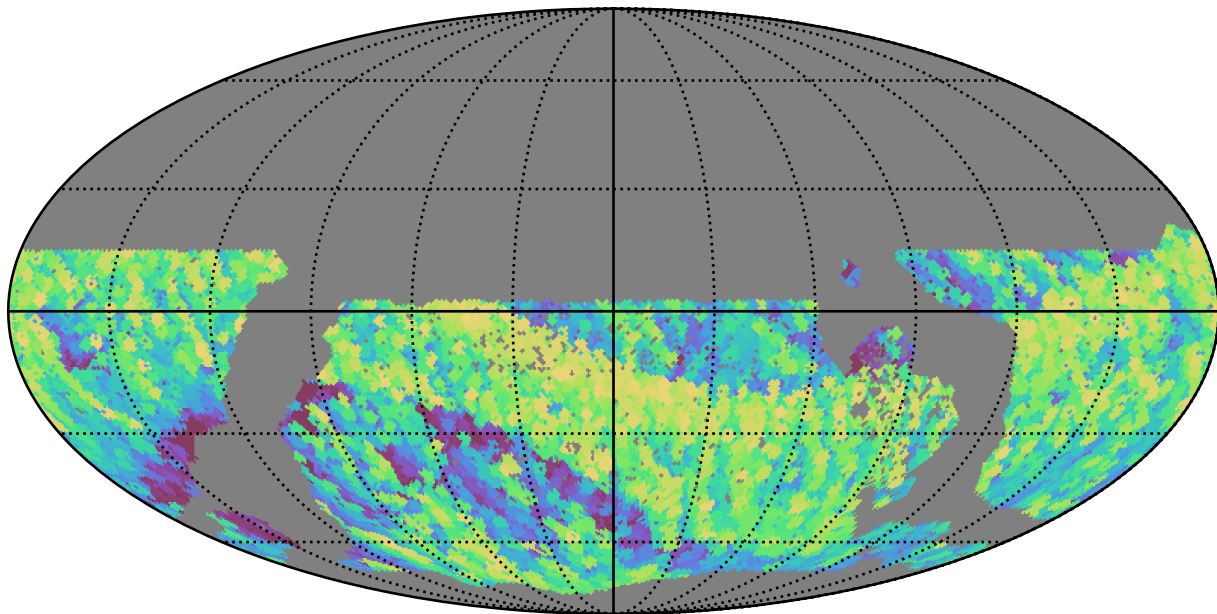
reweight_plane_v3.3_10yrs WFD z band: Max airmass
