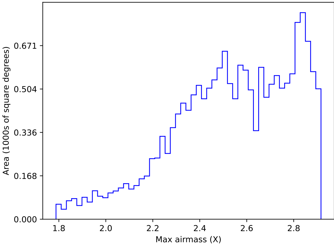
reweight_plane_v3.3_10yrs WFD z band: Max airmass
