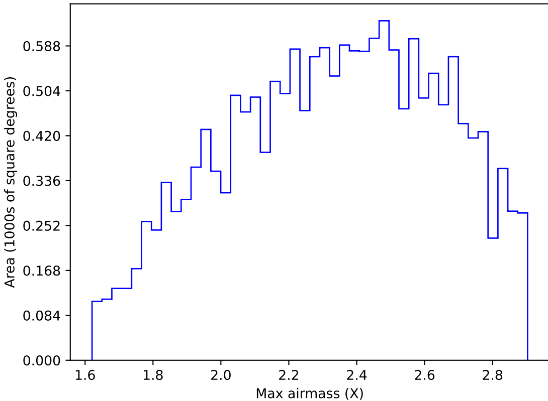
reweight_plane_v3.3_10yrs WFD y band: Max airmass
