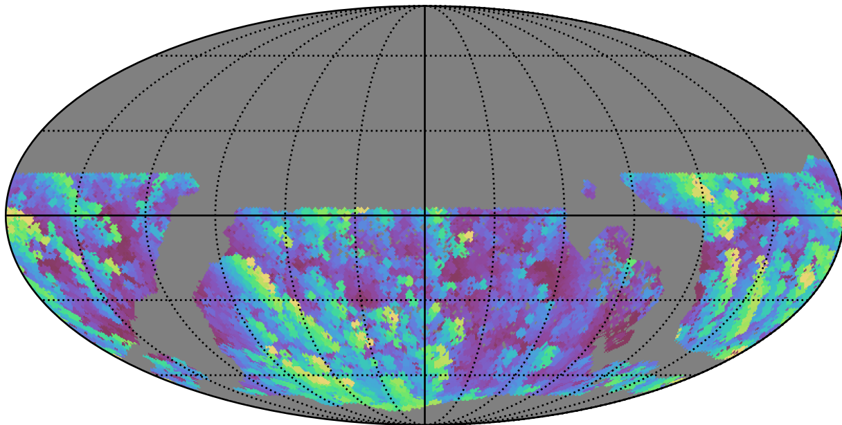
reweight_plane_v3.3_10yrs WFD u band: Max airmass
