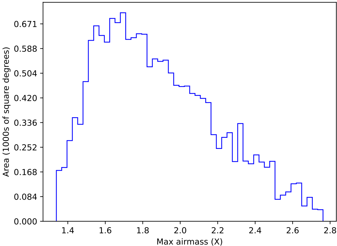
reweight_plane_v3.3_10yrs WFD u band: Max airmass
