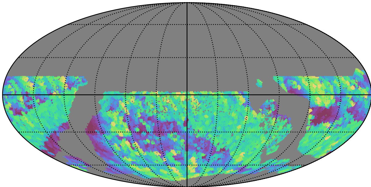
reweight_plane_v3.3_10yrs WFD r band: Max airmass
