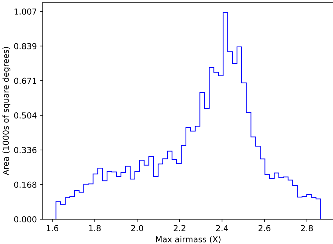
reweight_plane_v3.3_10yrs WFD r band: Max airmass
