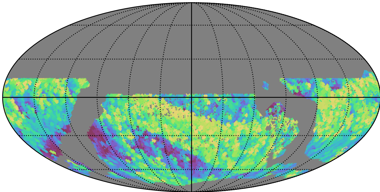
reweight_plane_v3.3_10yrs WFD i band: Max airmass
