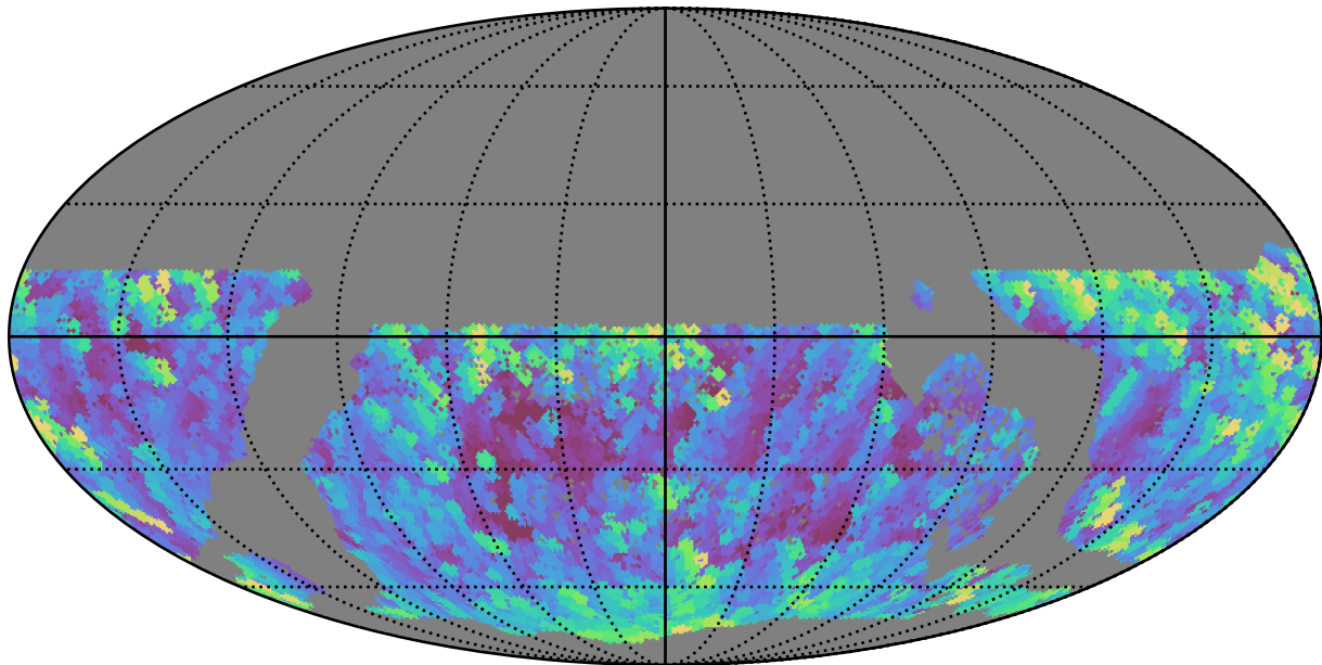
reweight_plane_v3.3_10yrs WFD g band: Max airmass
