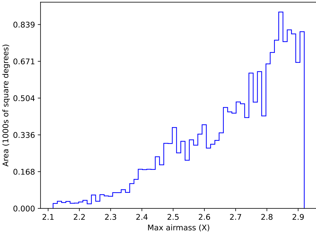
reweight_plane_v3.3_10yrs WFD all bands: Max airmass
