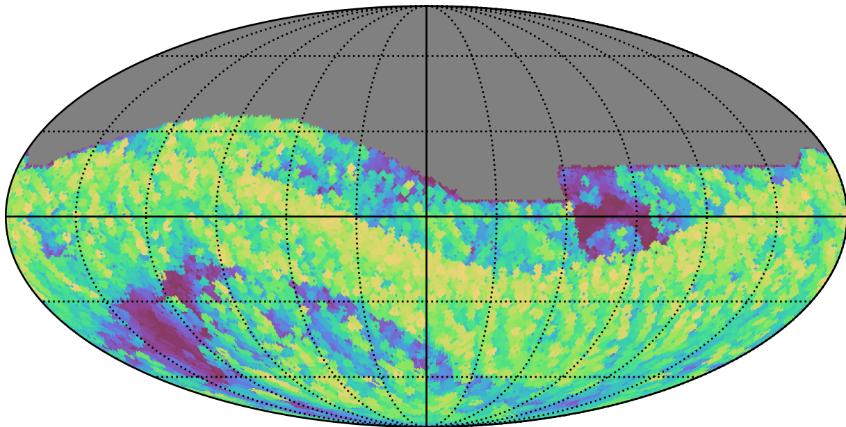
reweight_plane_v3.3_10yrs All sky z band: Max airmass
