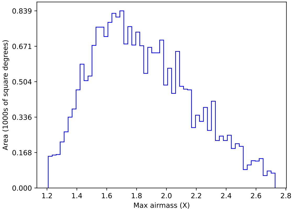
reweight_plane_v3.3_10yrs All sky u band: Max airmass
