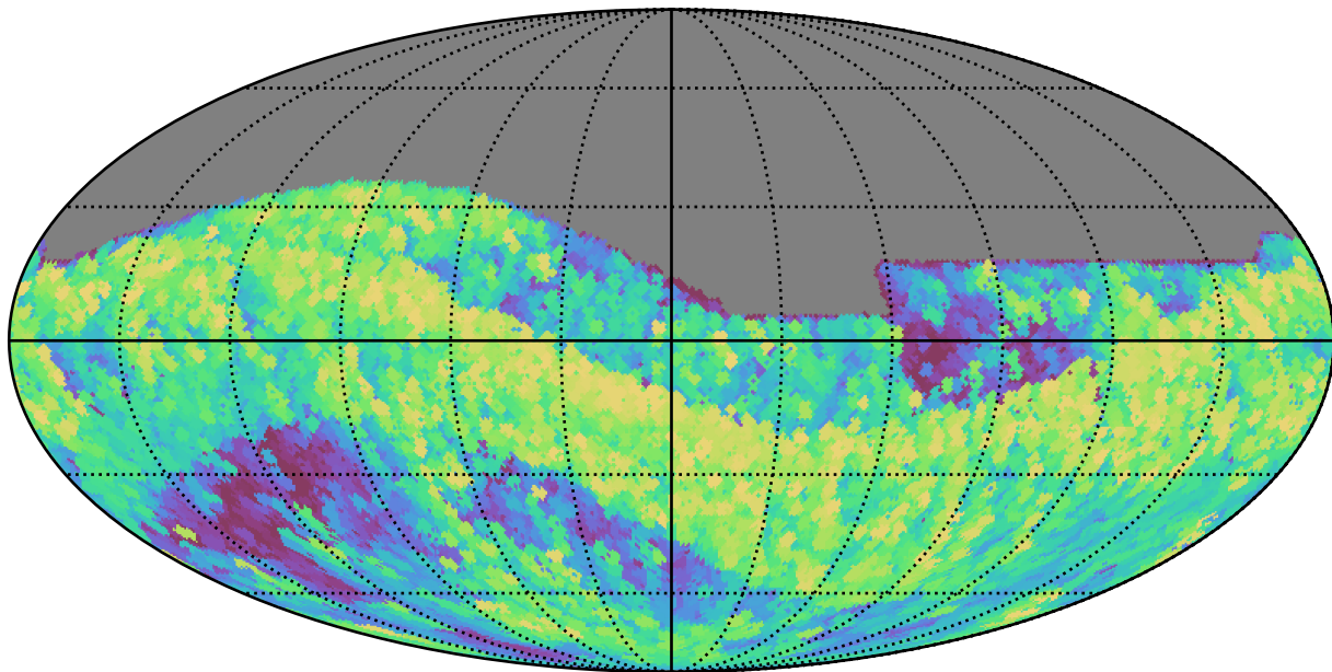
reweight_plane_v3.3_10yrs All sky i band: Max airmass
