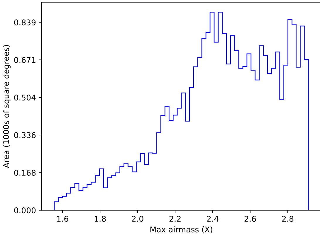
reweight_plane_v3.3_10yrs All sky i band: Max airmass
