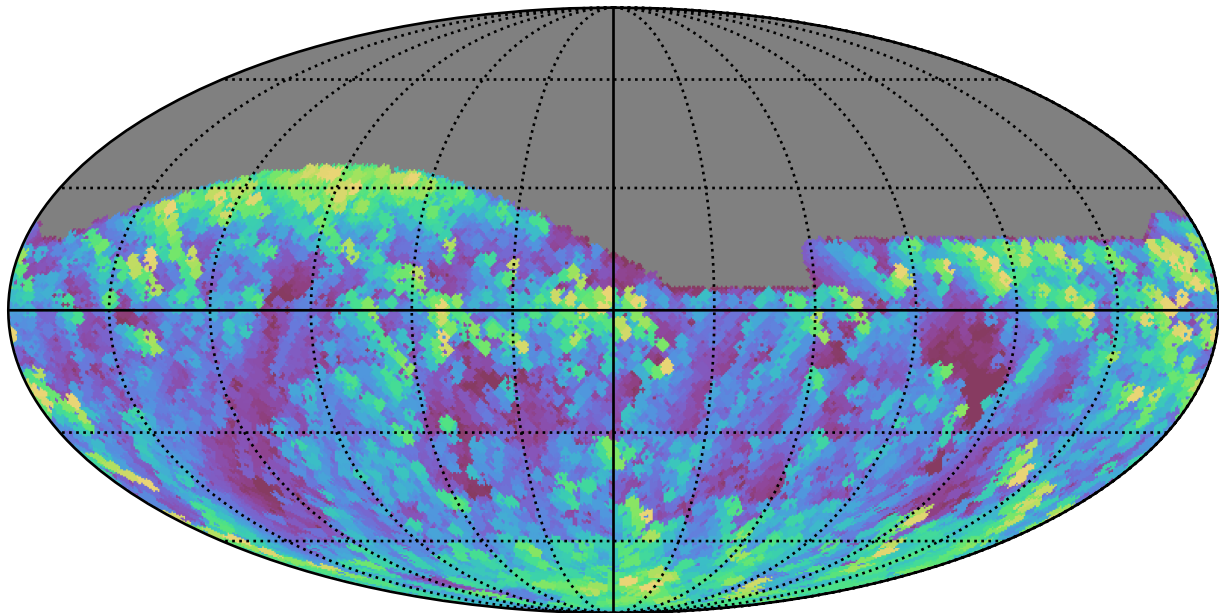
reweight_plane_v3.3_10yrs All sky g band: Max airmass
