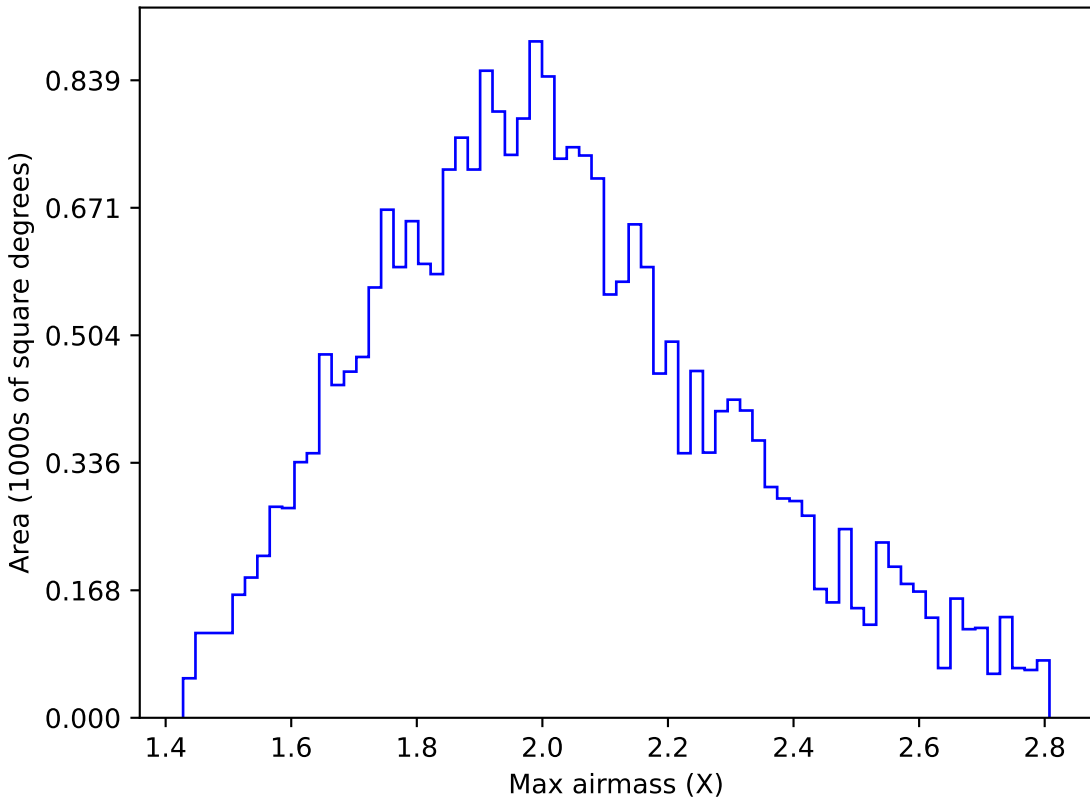
reweight_plane_v3.3_10yrs All sky g band: Max airmass
