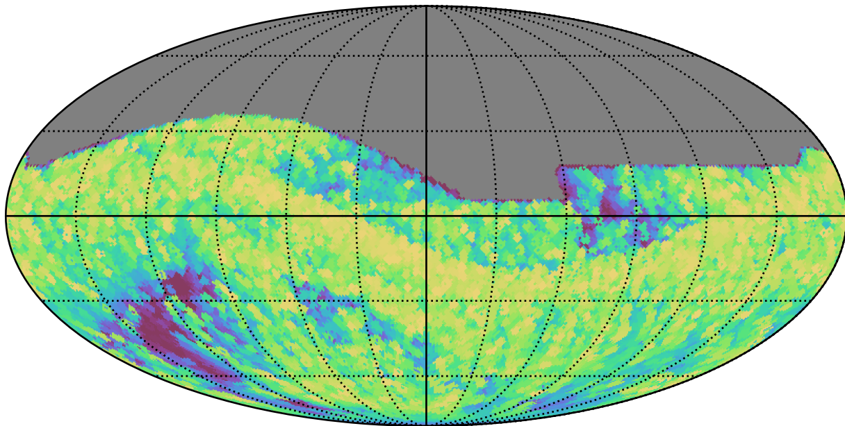
reweight_plane_v3.3_10yrs All sky all bands: Max airmass
