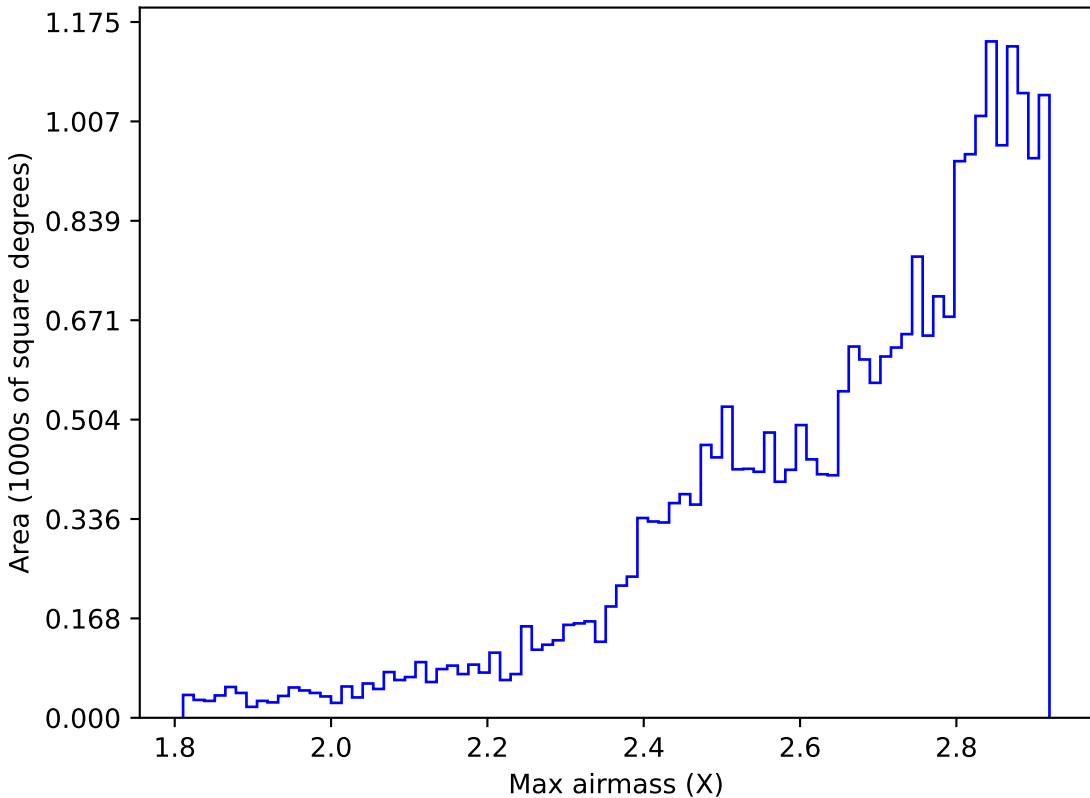
reweight_plane_v3.3_10yrs All sky all bands: Max airmass
