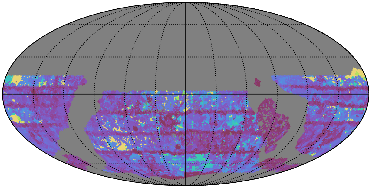
reweight_plane_v3.3_10yrs WFD z band: Max Inter-Night Gap
