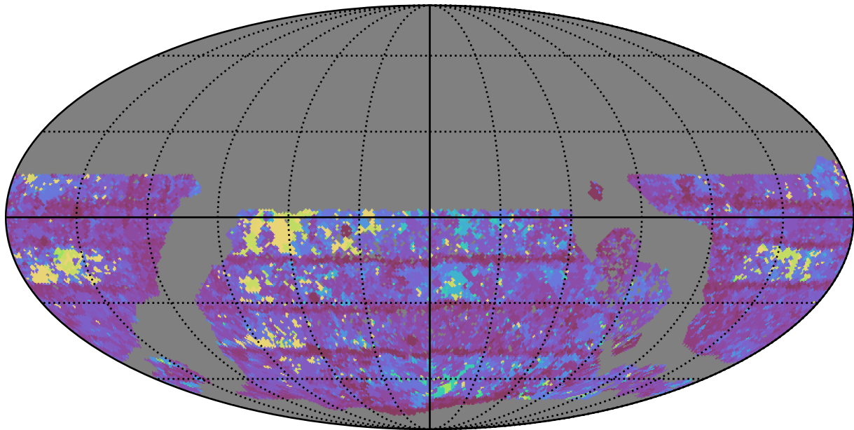
reweight_plane_v3.3_10yrs WFD y band: Max Inter-Night Gap
