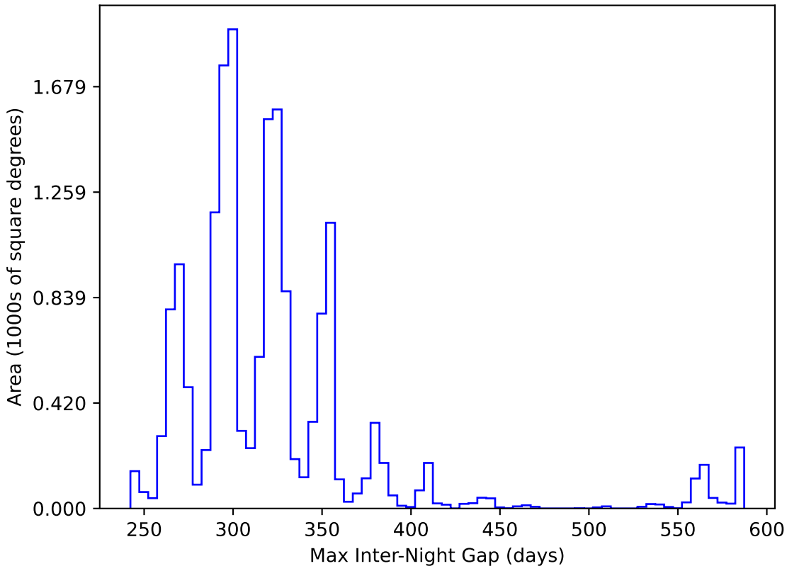
reweight_plane_v3.3_10yrs WFD y band: Max Inter-Night Gap
