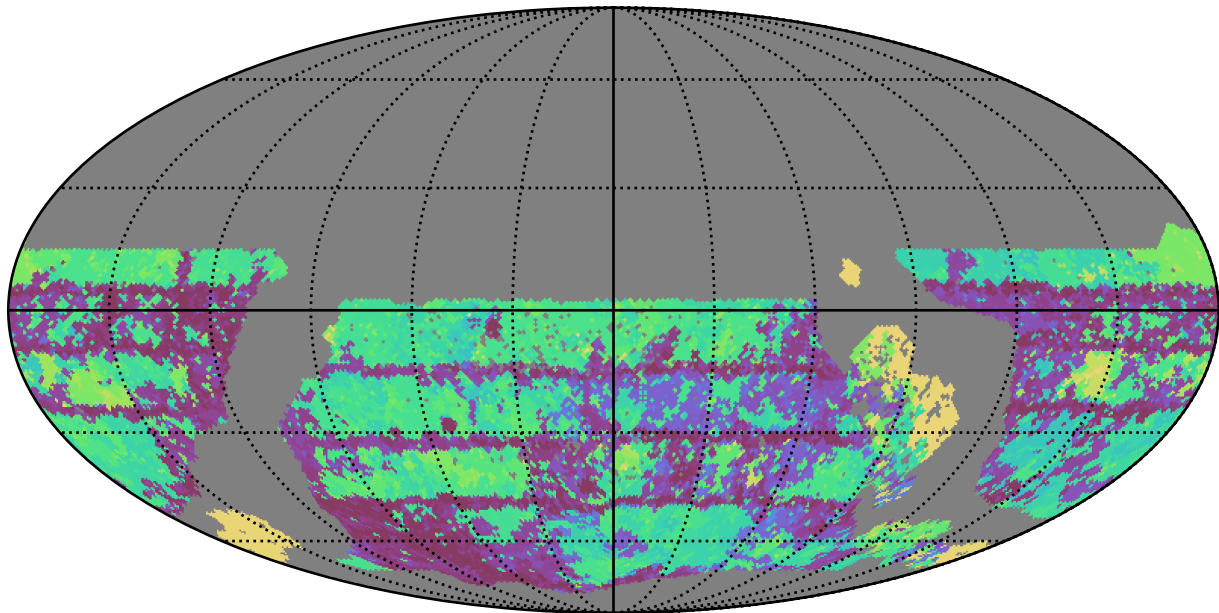
reweight_plane_v3.3_10yrs WFD u band: Max Inter-Night Gap
