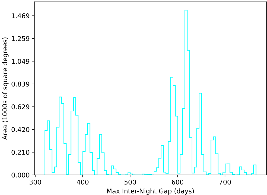
reweight_plane_v3.3_10yrs WFD u band: Max Inter-Night Gap
