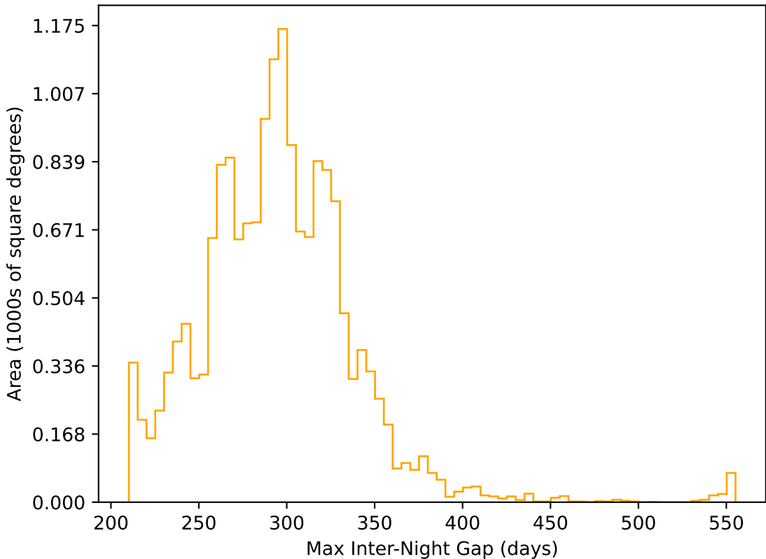
reweight_plane_v3.3_10yrs WFD r band: Max Inter-Night Gap
