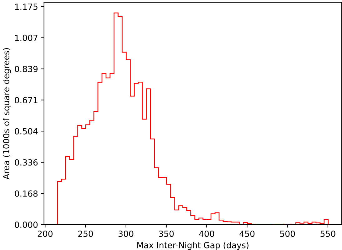
reweight_plane_v3.3_10yrs WFD i band: Max Inter-Night Gap
