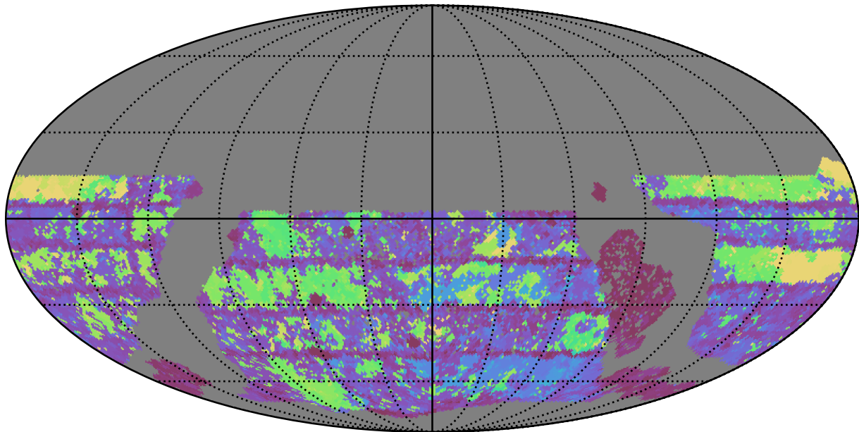
reweight_plane_v3.3_10yrs WFD g band: Max Inter-Night Gap
