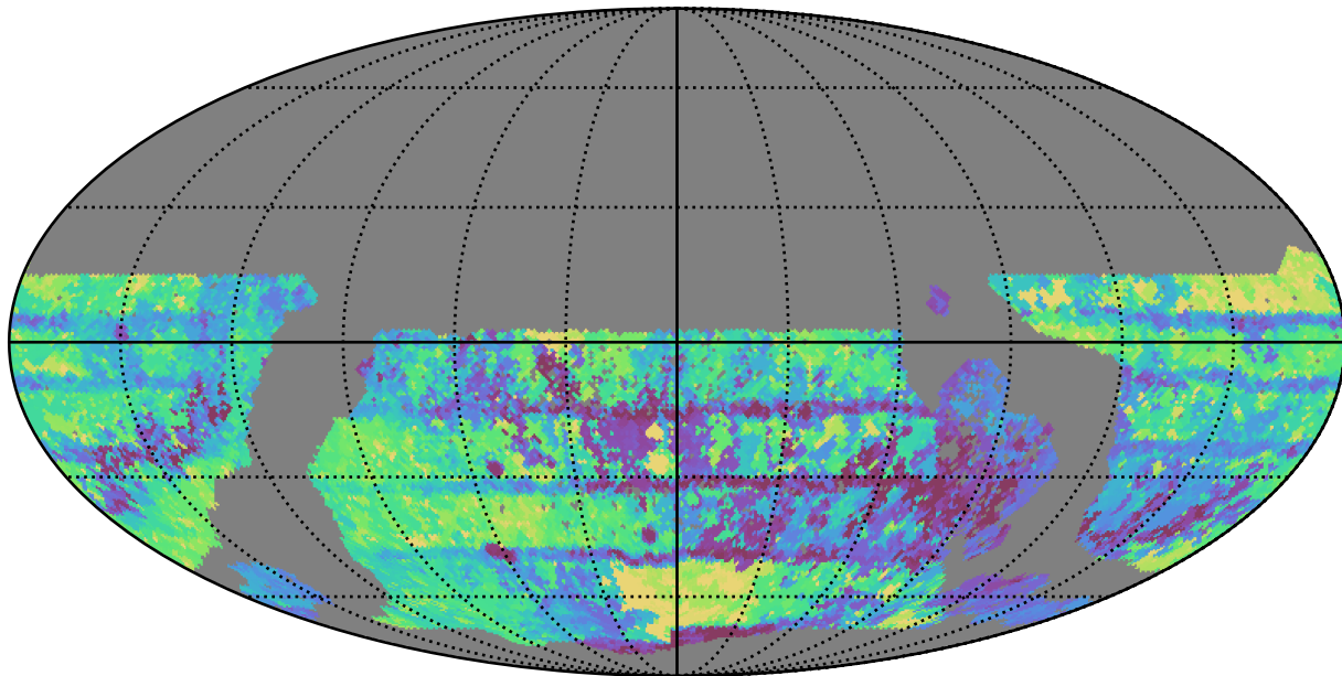
reweight_plane_v3.3_10yrs WFD all bands: Max Inter-Night Gap
