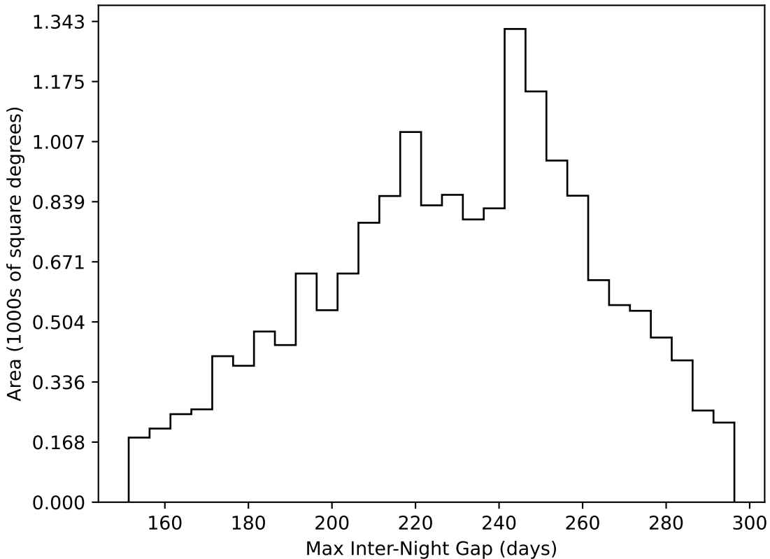
reweight_plane_v3.3_10yrs WFD all bands: Max Inter-Night Gap
