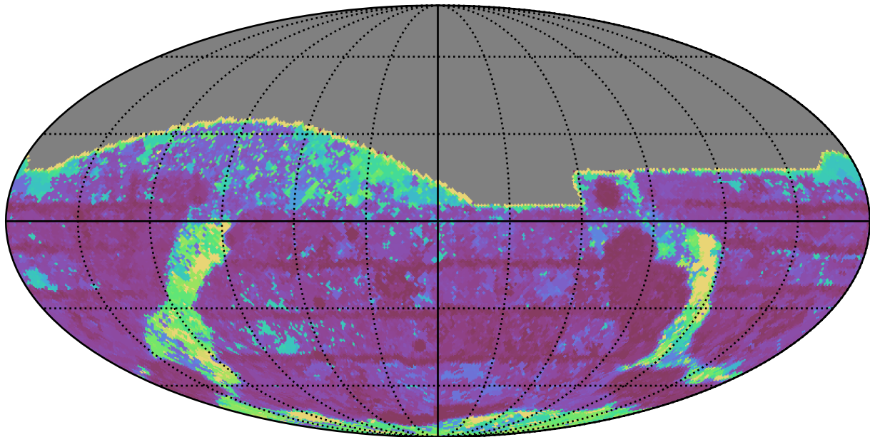
reweight_plane_v3.3_10yrs All sky z band: Max Inter-Night Gap
