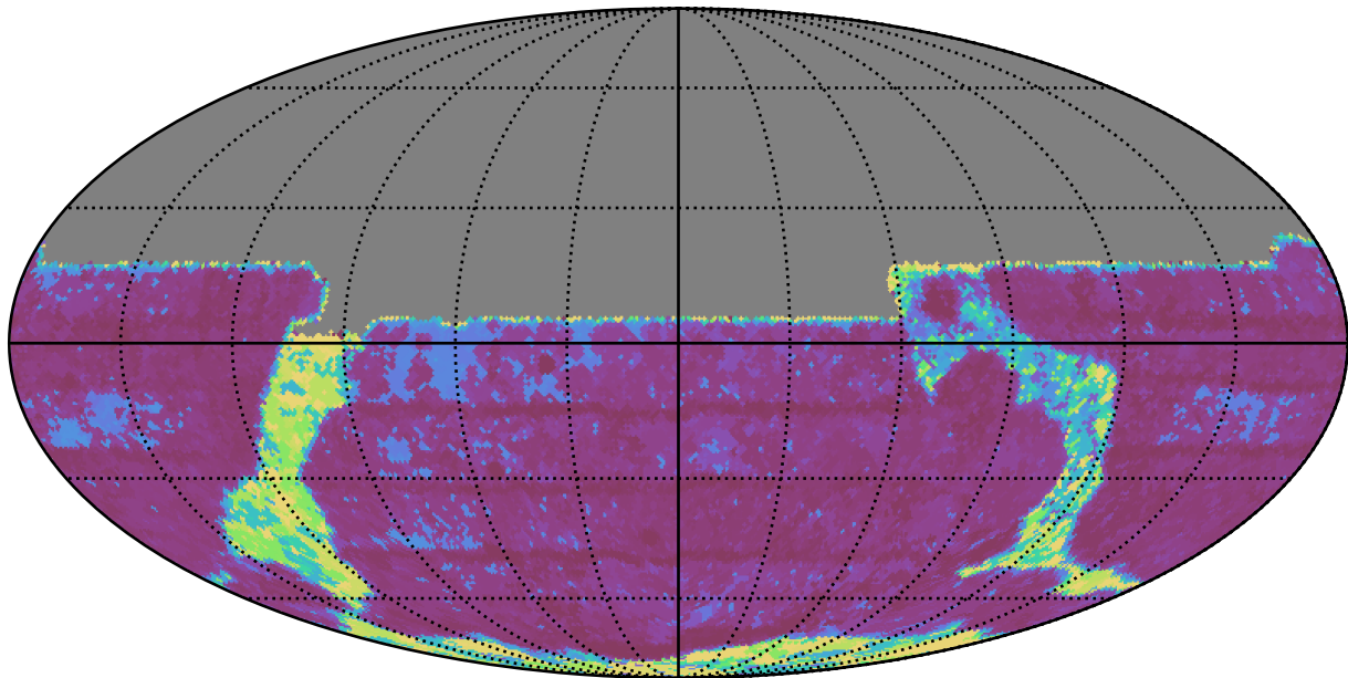
reweight_plane_v3.3_10yrs All sky y band: Max Inter-Night Gap
