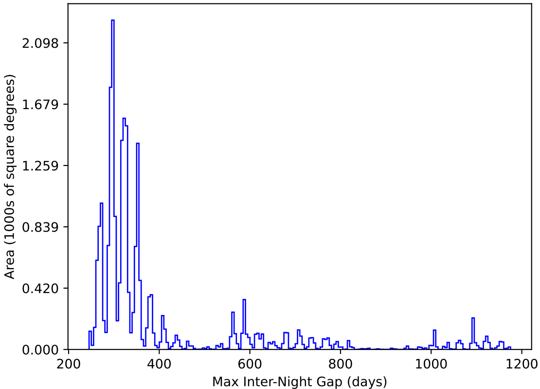
reweight_plane_v3.3_10yrs All sky y band: Max Inter-Night Gap
