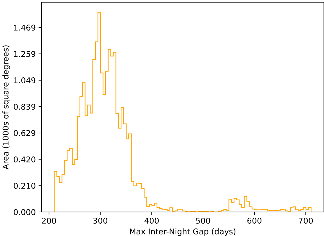
reweight_plane_v3.3_10yrs All sky r band: Max Inter-Night Gap
