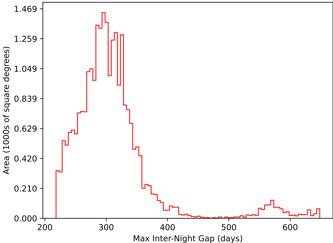
reweight_plane_v3.3_10yrs All sky i band: Max Inter-Night Gap
