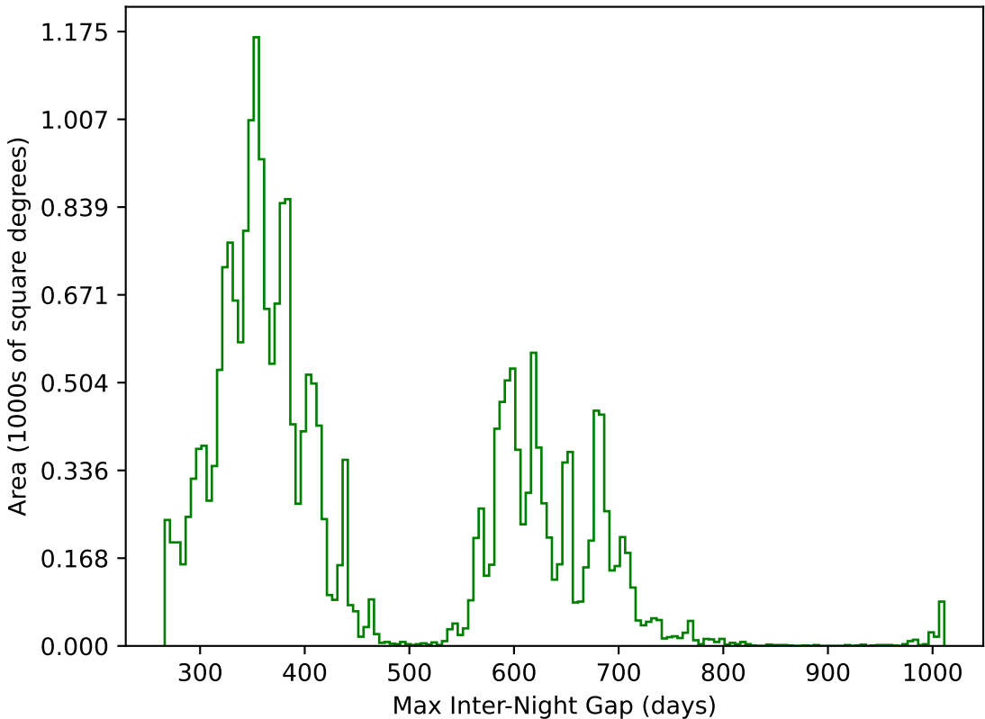
reweight_plane_v3.3_10yrs All sky g band: Max Inter-Night Gap
