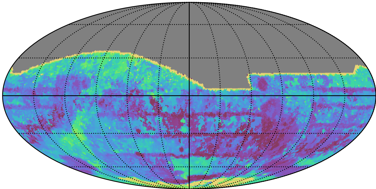
reweight_plane_v3.3_10yrs All sky all bands: Max Inter-Night Gap
