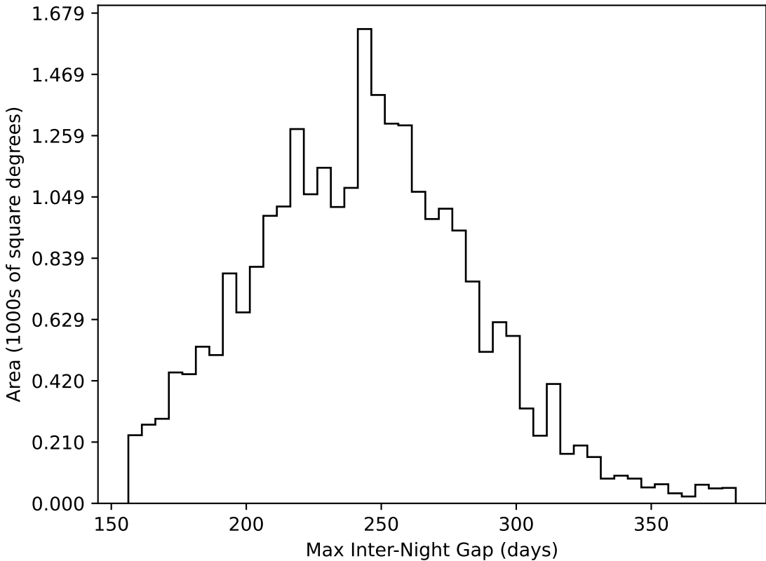
reweight_plane_v3.3_10yrs All sky all bands: Max Inter-Night Gap
