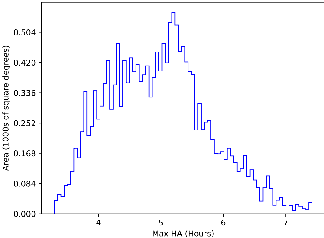
reweight_plane_v3.3_10yrs WFD z band: Max HA
