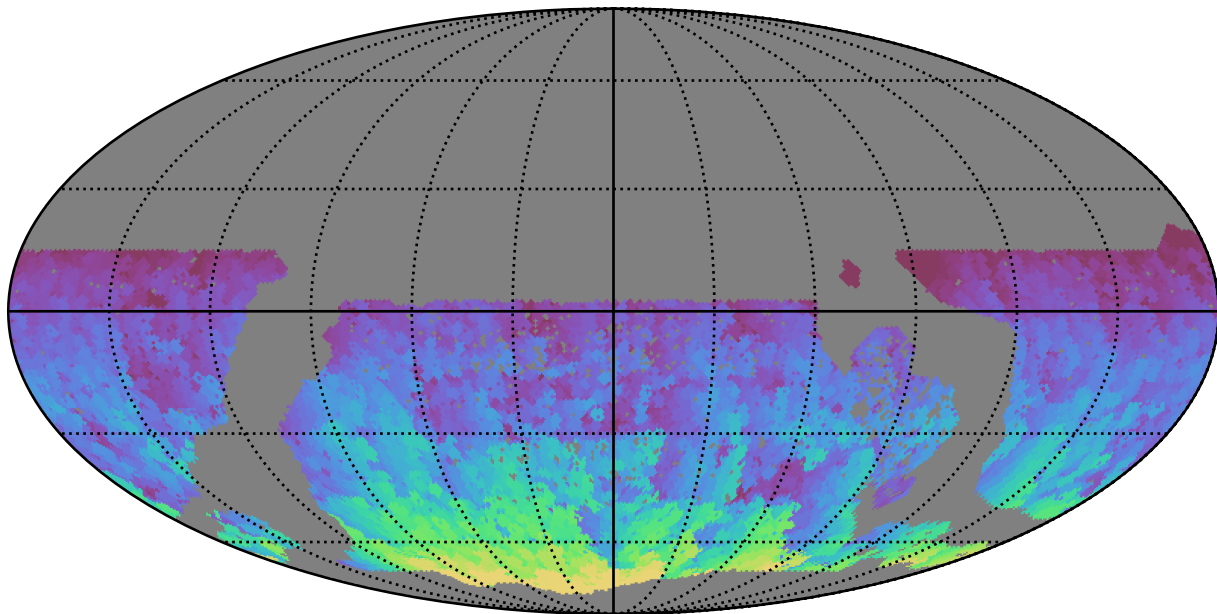
reweight_plane_v3.3_10yrs WFD y band: Max HA
