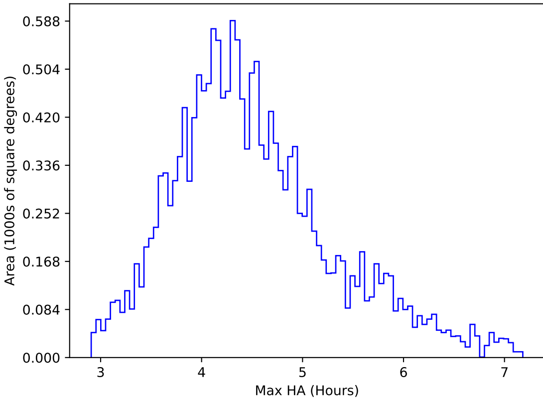
reweight_plane_v3.3_10yrs WFD r band: Max HA
