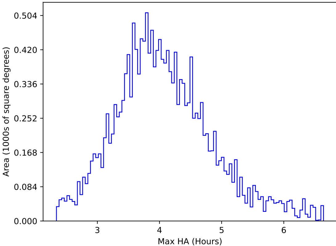
reweight_plane_v3.3_10yrs WFD g band: Max HA
